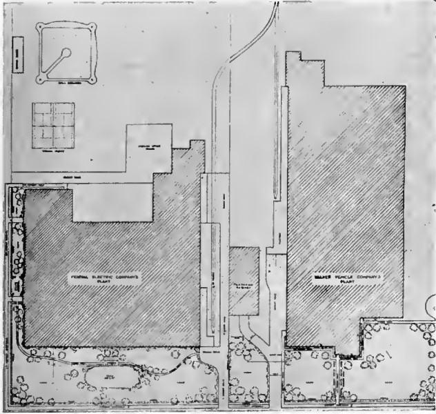
PLAN OF GROUNDS OF BUILDINGS FOR WALKER VEHICLE CO. AND FEDERAL ELECTRIC CO.
